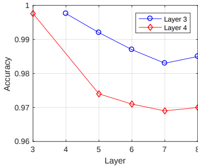
Figure 10.11: Recognition accuracy of combinations of layer 3 and 4 with layers [3, ..., 8].
