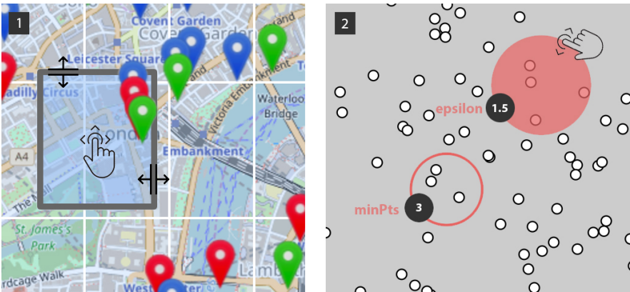
Figure 3.2: In 2.1: the draggable and resizable widget to select a specific area on the map. In 2.2: \epsilon and minPts of DBSCAN can be defined dragging the circles' circumference on a distribution of points.
